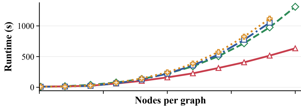
Plain networks
