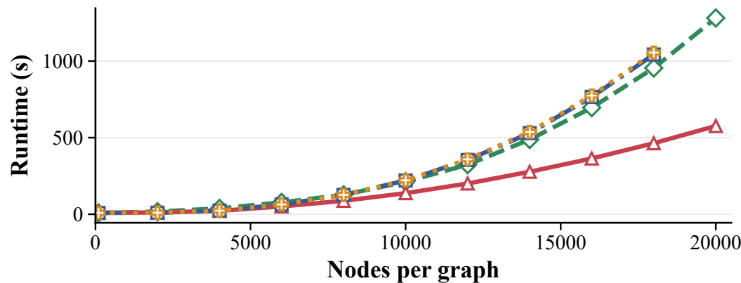
Attributed networks
